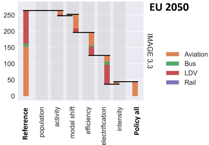
CO2-Emissions Transport [MtCO2]
